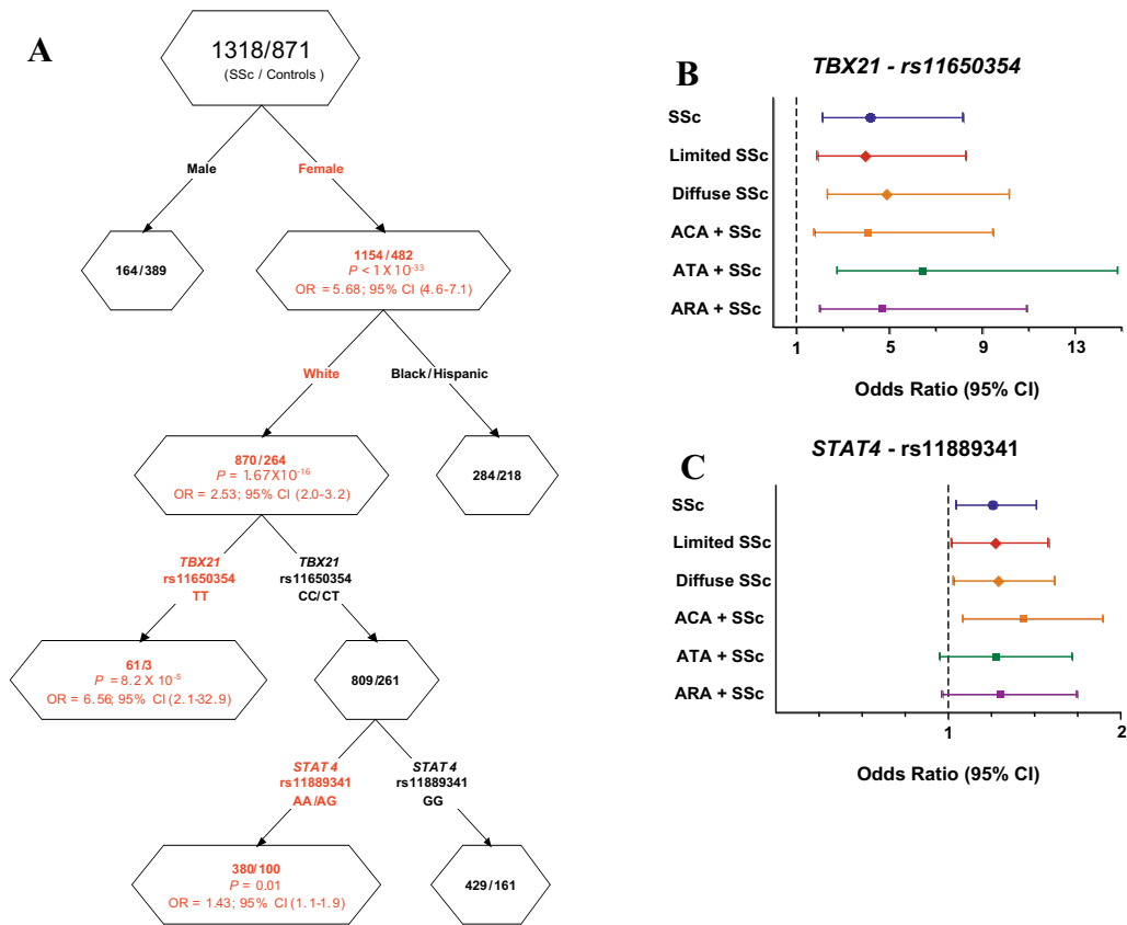
Figure 1. A, Cartesian and Regression Tree analysis showing a gene-gene interaction between TBX21 and STAT4 polymorphisms in systemic sclerosis (SSc). Red text denotes SSc susceptibility factors. B and C, Estimated risk of TBX21 single-nucleotide polymorphism (SNP) rs11650354 (B) and STAT4 SNP rs11889341 (C) in SSc patients, by logistic regression analysis. The analysis was controlled for the confounding effects of sex and race. Control subjects were used as reference for all comparisons. The TBX21 SNP showed a recessive mode of inheritance, and the STAT4 SNP showed a dominant mode of inheritance. OR = odds ratio; 95% CI = 95% confidence interval; ACA = anticentromere antibody; ATA = anti-topoisomerase I antibody; ARA = anti-RNA polymerase III antibody.
