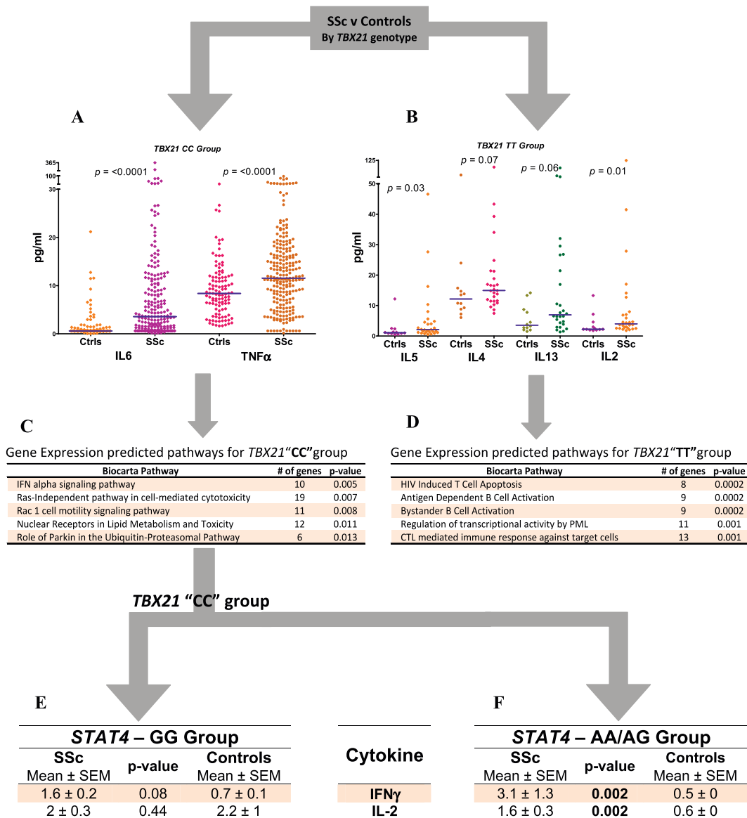
Figure 2. A–D, Plasma cytokine levels (A and B) and gene expression predicted pathways (C and D) by TBX21 single-nucleotide polymorphism (SNP) group in systemic sclerosis (SSc) patients compared with healthy controls (Ctrls). Bars in A and B show the means. P values for gene expression predicted pathways were determined by Fisher’s least significant statistic after 100,000 permutations ( http://cgap.nci.nih.gov/Pathways/BioCarta/ ). E and F, Gene expression predicted pathways by STAT4 SNP group in SSc patients compared with healthy controls. IL-6 = interleukin-6; TNF \alpha = tumor necrosis factor \alpha ; IFN = interferon; HIV = human immunodeficiency virus; PML = promyelocytic leukemia; CTL = cytotoxic T lymphocyte.
